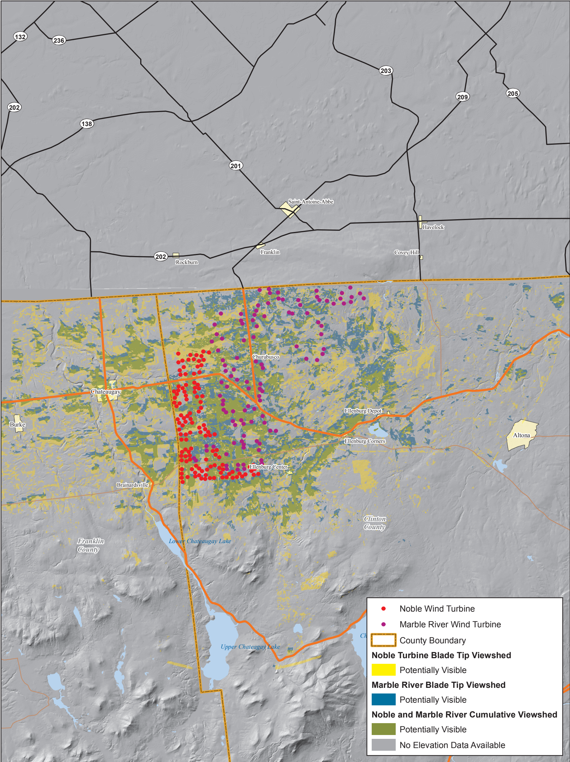
Figure 6: Viewshed Analysis Blade Tip (399 ft.) Topography & Vegetation Noble & Marble River Cumulative Viewshed Sheet 6 of 6 Marble River Wind Farm Towns of Clinton and Ellenburg Clinton County, New York
