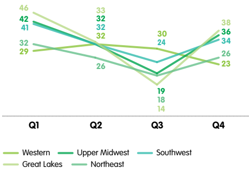
EDPR NA 2009 Quarterly Load Factors (%)
