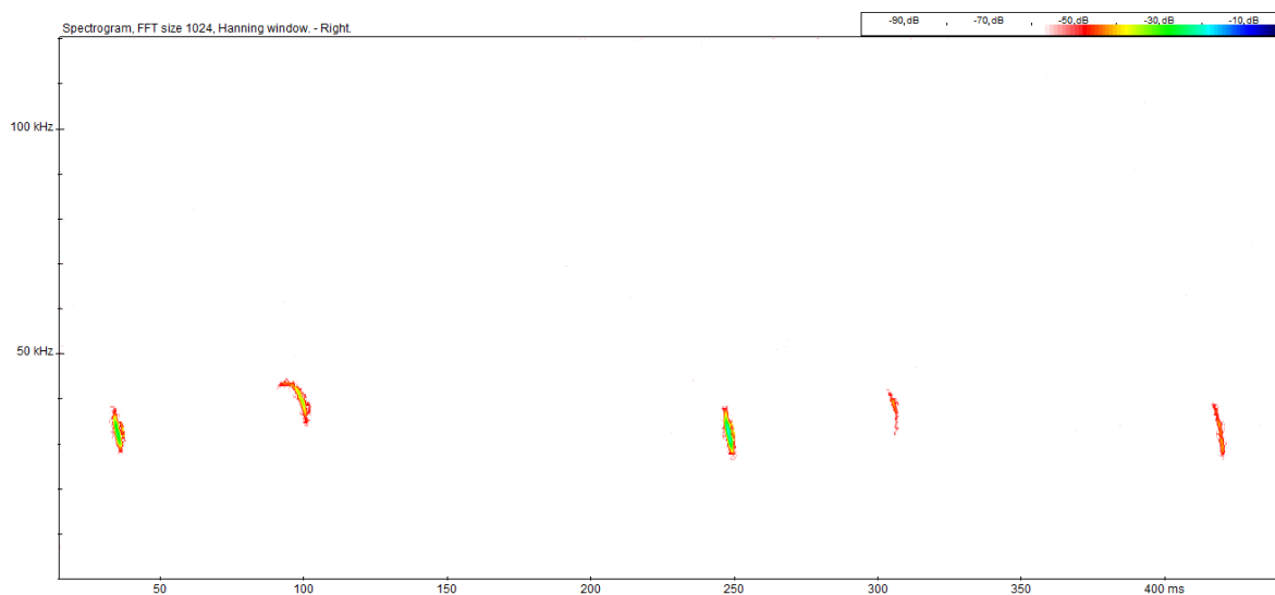
Figura III.11 Barbastella barbastellus , 20.06.2014, wav 163, punct 3
